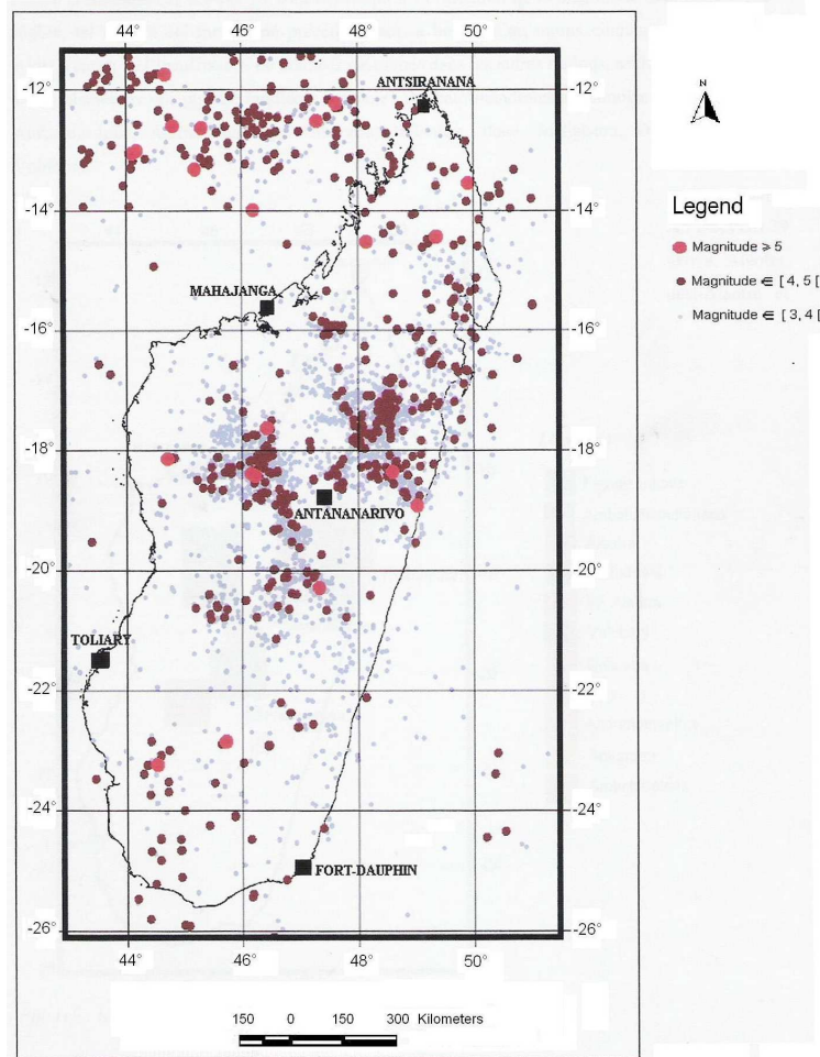
Figure 2: Instrumental seismic activity for the period 1975-2007 for magnitude \geq 3 (Rindraharisaona, 2008)
