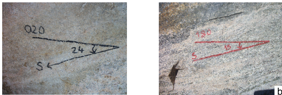
Figure 6: Field photographs showing close-up views of slickenside with a rake of up to 24° on the fault segment comprising the Lac Andranomena fault set
