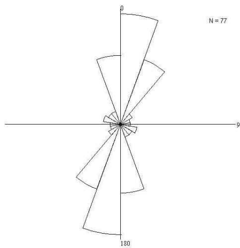
Figure 8: Rose diagram of major fracture orientations: numbers and lengths
